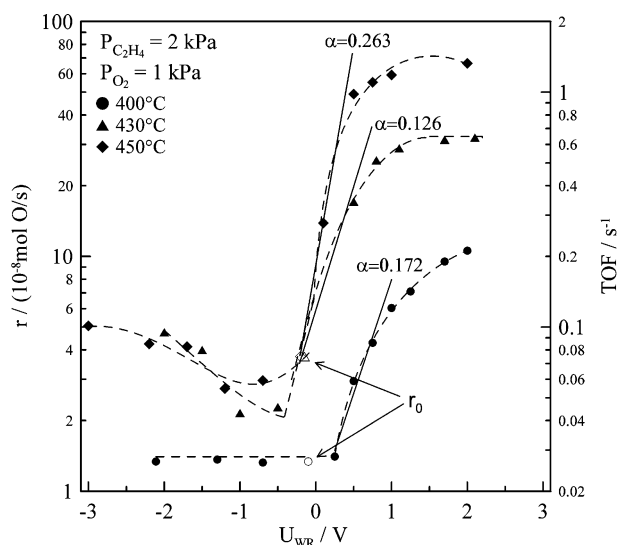
Figure 4. Effect of catalyst potential on the rate of C 2 H 4 oxidation on RuO 2 /YSZ.
