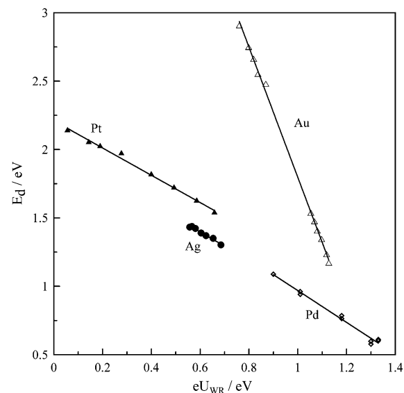
Figure 13. Effect of catalyst potential on the oxygen desorption activation energy, E_d , calculated from the modified Redhead analysis of O 2 TPD spectra from Pt, Ag, Au and Pd electrodes deposited on YSZ [14,42].
