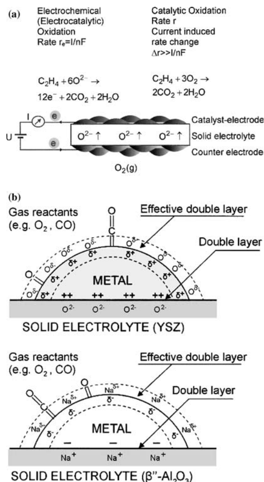
Figure 1. (a) Principle and basic experimental setup for electrochemical promotion (NEMCA) studies using an \text{O}^{2-} -conducting solid electrolyte. (b) Schematic representation of a metal catalyst-electrode deposited on an \text{O}^{2-} -conducting electrolyte and a \text{Na}^+ -conducting solid electrolyte, showing the location of the metal-solid electrolyte double layer and of the effective double layer created at the metal/gas interface due to potential-controlled ion migration (backspillover).
